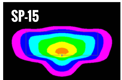
General optics for roads with very long pole spacing. Offers even light also in wet conditions. Relatively wide road profile (lits also opposite cycleways if the pole spacing is short)
