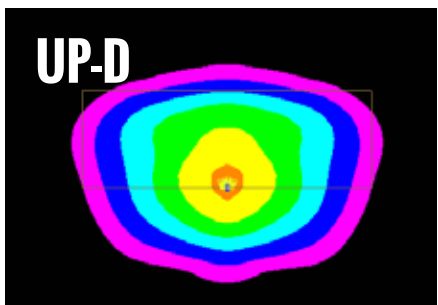
Road/area optics for short pole spacing. Offers a lot of back area light.
